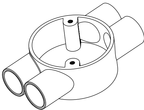
Isometric view
